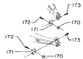
40-603 90° BLADE HOLDER
